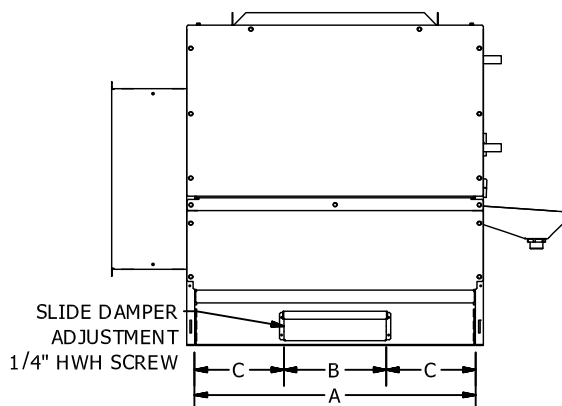
MANUAL DAMPER OPTION
