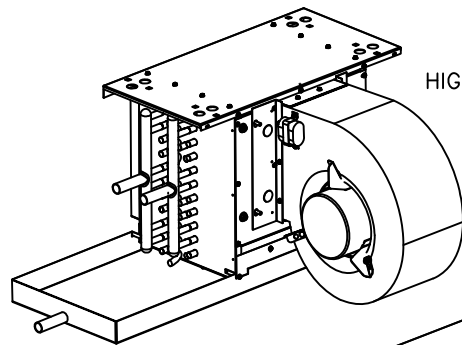
MODEL "KHGP" HIGH PERFORMANCE PLENUM RETURN FAN COIL UNIT
