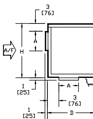
BOT/REAR INLET
