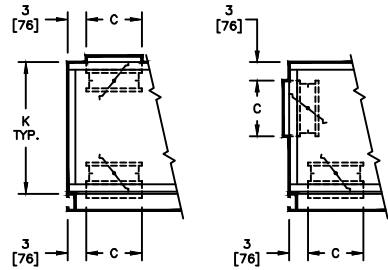
TOP/RTM INLET
