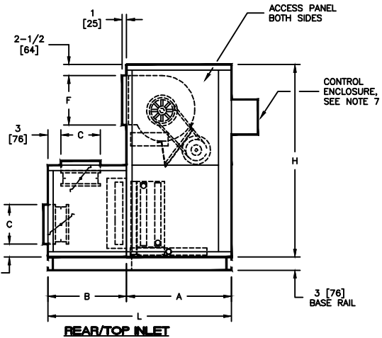
REAR/TOP INLET
