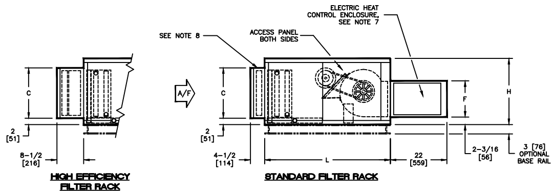
SIDE VIEWS
