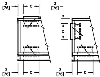
TOP/BTM INLET
