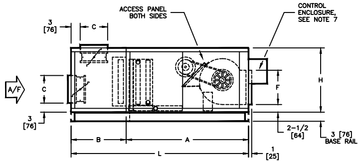
REAR/TOP INLET
