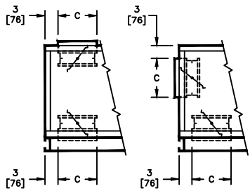
TOP/BTM INLET
