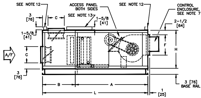
REAR/TOP INLET
