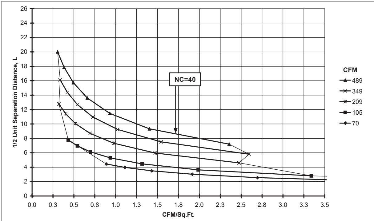
DIFFUSER SPACING FOR 80% ADPI: PLQIMP, 24"x24" PANEL, 8" NECK, 4-WAY (NO DAMPER)
