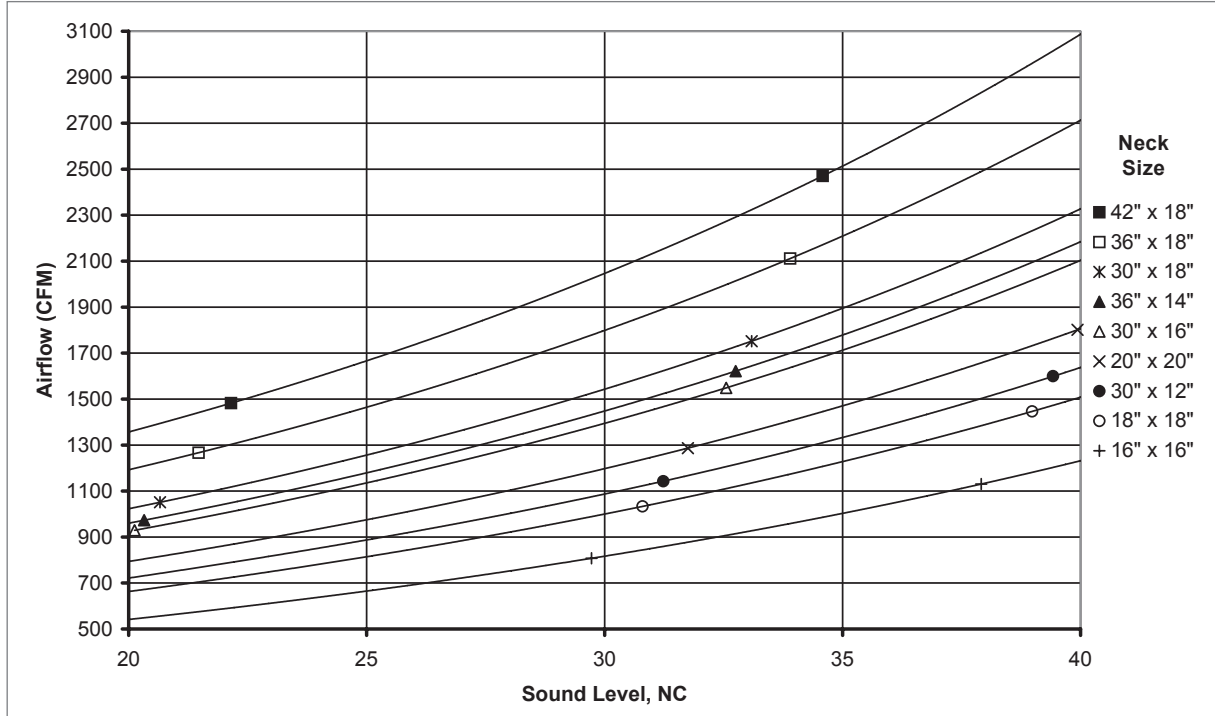
AIRFLOW VS. NC: S480, 38° DEFLECTION (NO DAMPER)
