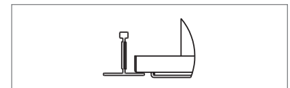
5RFHF, 9RFHF, 90° LAY-IN T-BAR
