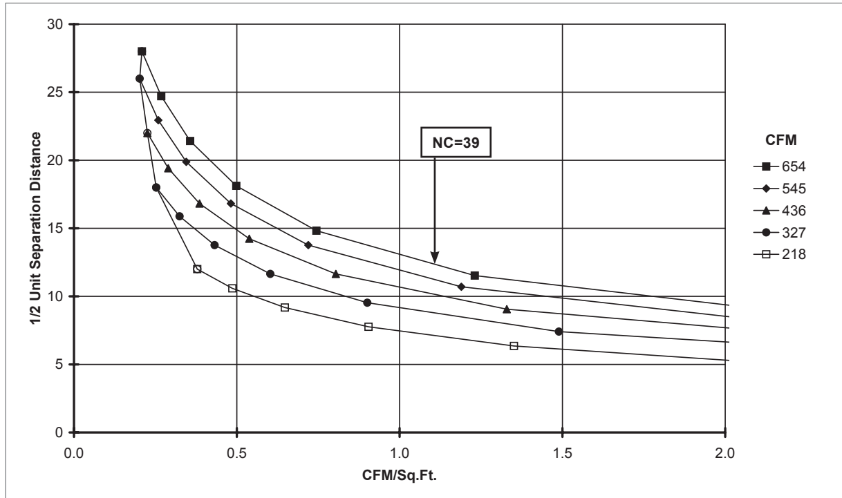
DIFFUSER SPACING FOR 80% ADPI: KSD, 10" NECK (NO DAMPER)
