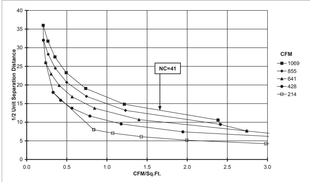
DIFFUSER SPACING FOR 80% ADPI: KSD, 14" NECK (NO DAMPER)
