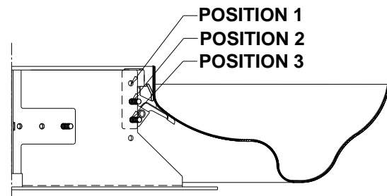
3-POSITION ADJUSTMENT PLAQUE SET AT POSITION 2
