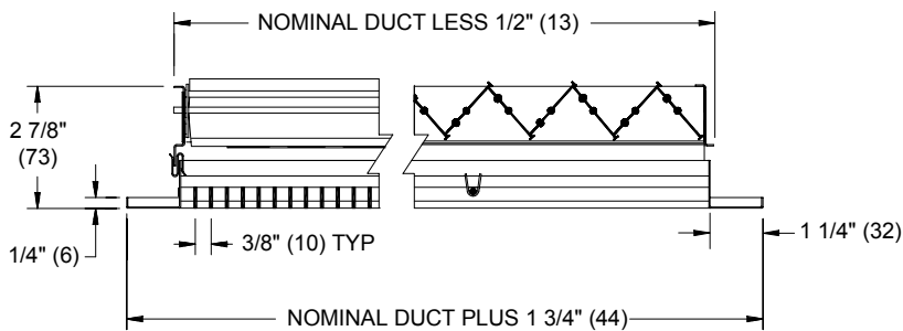
CENTER CROSS SECTION w/ OBD
