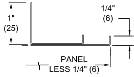
Frame 23 LAY-IN T-BAR
