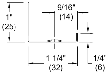
Frame 22 SURFACE MOUNT
