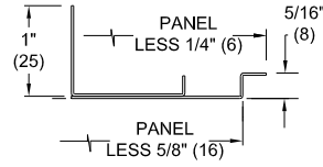
Frame 98 NARROW TEE
