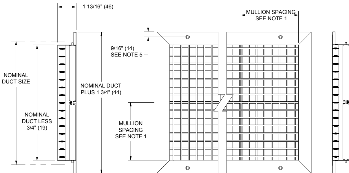
CENTER CROSS SECTION w/ OBD
