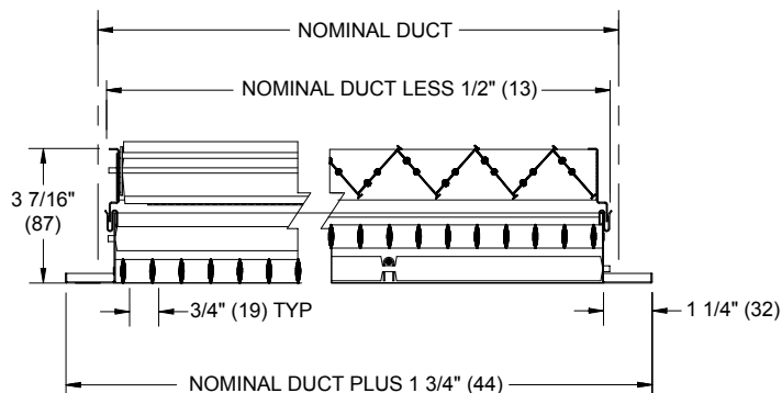
CENTER CROSS SECTION w/ OBD
