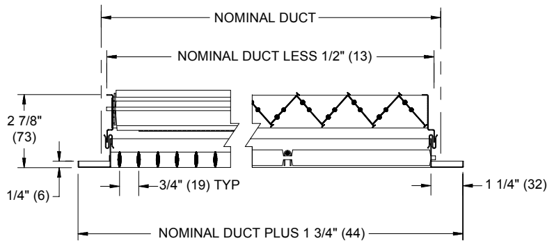
CENTER CROSS SECTION w/ OBD
