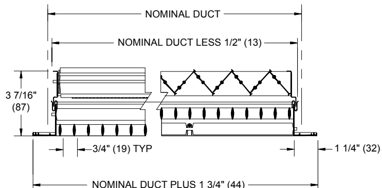
CENTER CROSS SECTION w/ OBD
