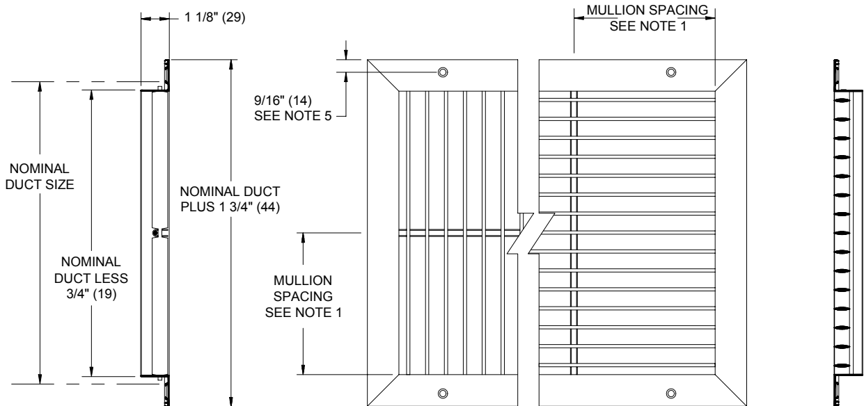
FACE VIEWS
