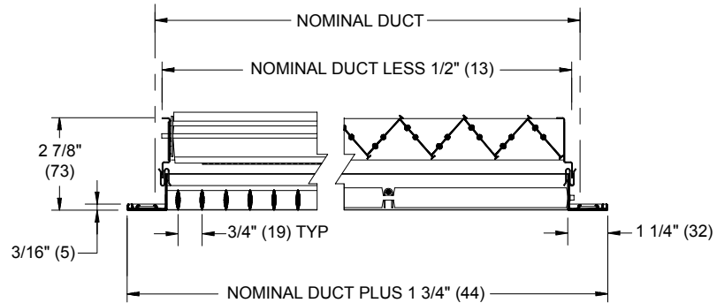
CENTER CROSS SECTIONS w/ OBD
