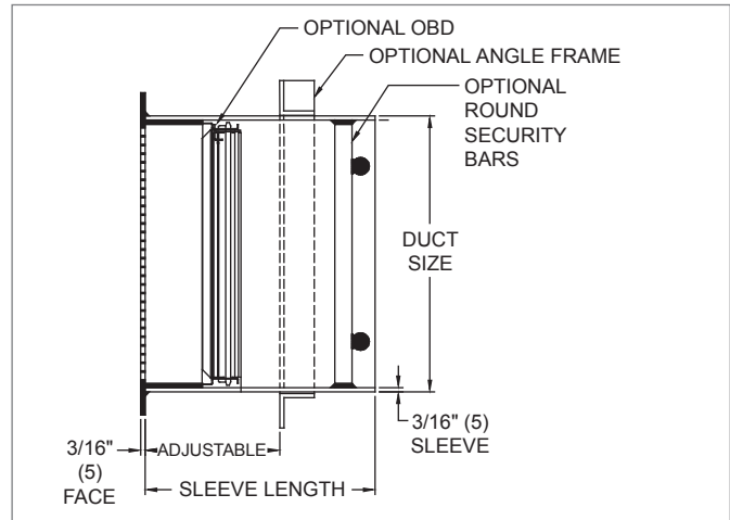
1310, CROSS SECTION
