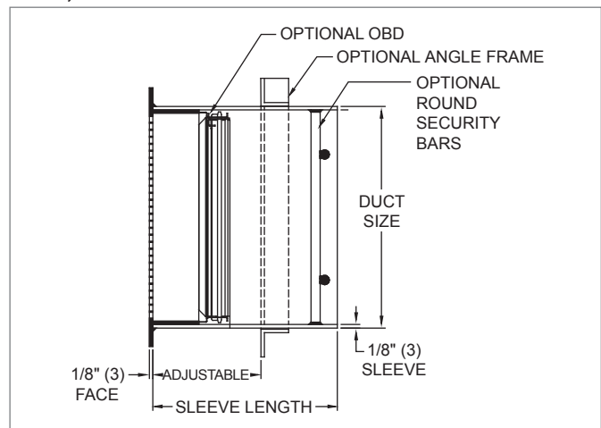
51310, CROSS SECTION
