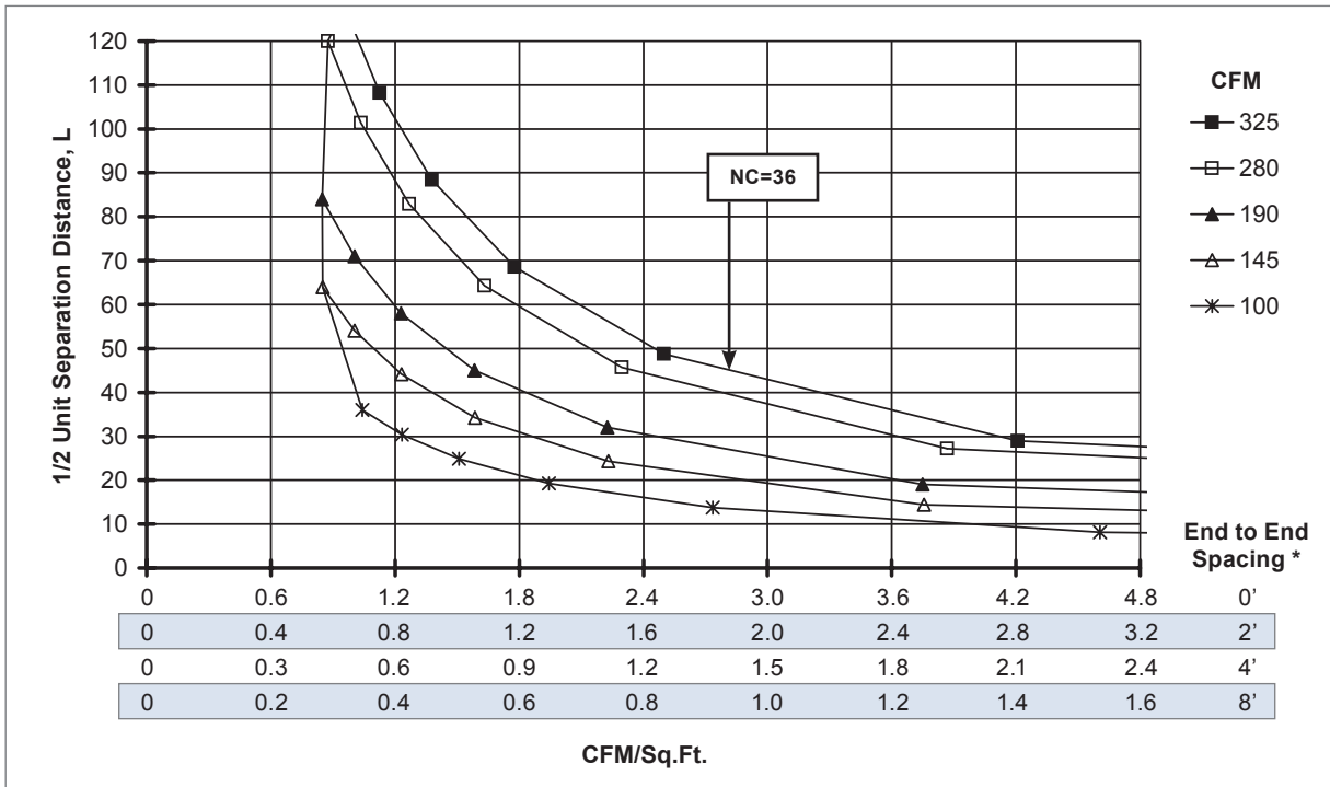
DIFFUSER SPACING FOR 80% ADPI: PTBSC, PTBSRC, 3/4" SLOT WIDTH, 4 FT., 1-SLOT, 8" OVAL INLET, 1-WAY (NO DAMPER)
