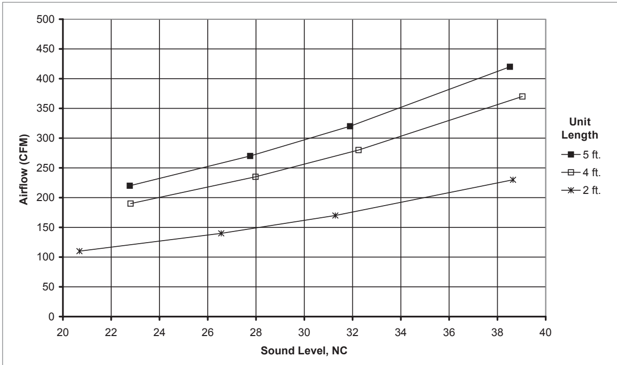
AIRFLOW VS. NC: PTBSC, PTBSRC, 3/4" SLOT WIDTH, 1-SLOT, 8" OVAL INLET, 1-WAY (NO DAMPER)
