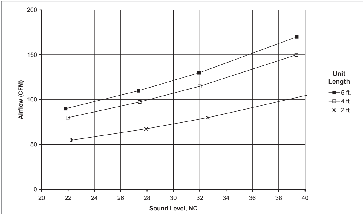
AIRFLOW VS. NC LEVEL: PTBS, 3/4" SLOT WIDTH, 1-SLOT, 8" OVAL INLET, 1-WAY (NO DAMPER)
