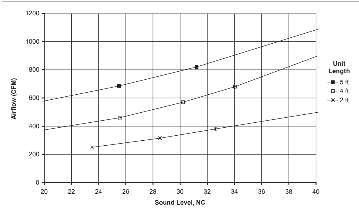
AIRFLOW VS. NC LEVEL: PTBR/PFTBR, 1" SLOT WIDTH, 2-SLOT (NO DAMPER)
