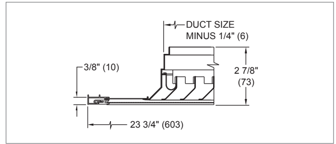
51240P, FRAME 23, LAY-IN T-BAR
