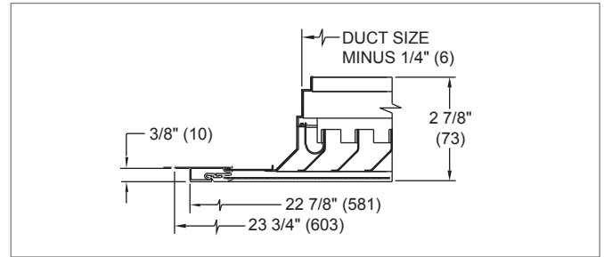
51240P, FRAME 30, DROP FACE
