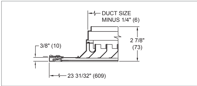
51240P, FRAME 29, CAMLOCK
