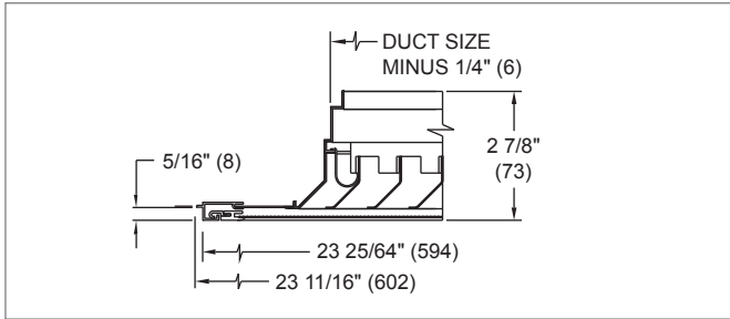
51240P, FRAME 98, NARROW-T
