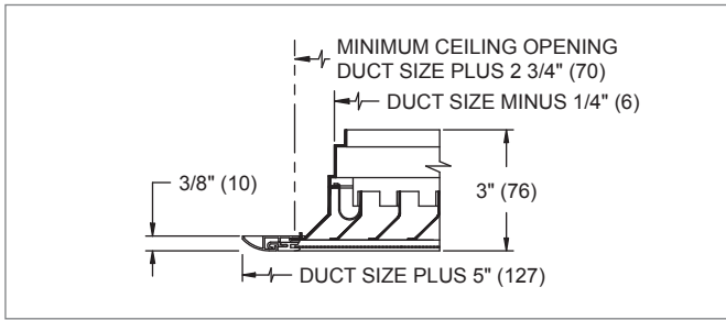
51240P, FRAME 22, SURFACE MOUNT
