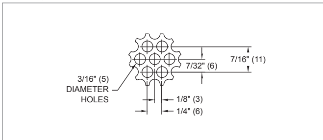
51240P, PERFORATION DETAIL
