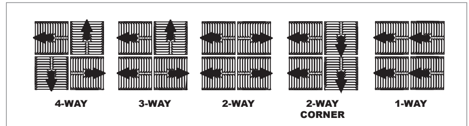
6600FR, DISCHARGE AIR PATTERNS
