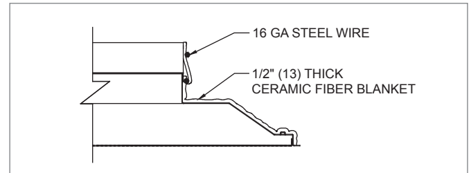
6600FR, FIRE BLANKET DETAIL
