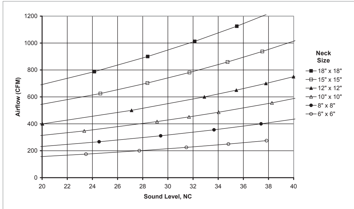
AIRFLOW VS. NC LEVEL: 6400, 56400, 24"x24" PANEL (NO DAMPER)
