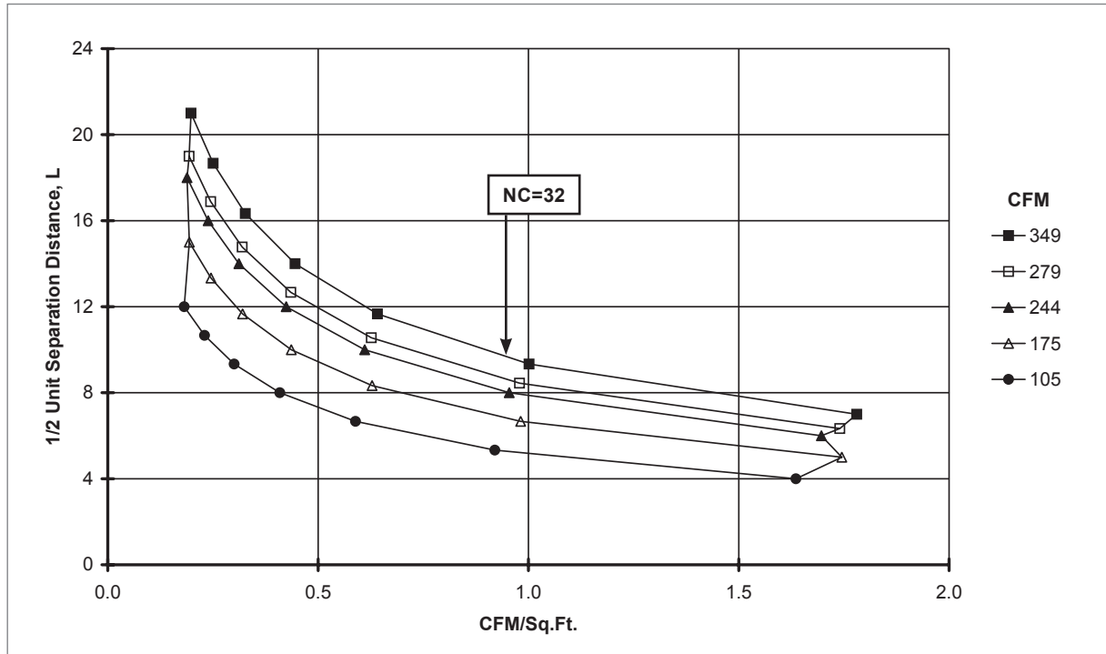
SPACING FOR 80% ADPI: 6500, 56500, 24"x24" PANEL, 8" NECK, 4-WAY (NO DAMPER)
