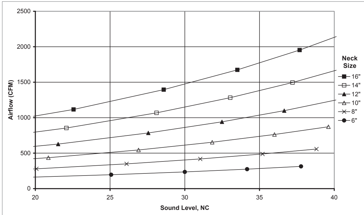
AIRFLOW VS. NC LEVEL: SHPCR, 5SHPCR (NO DAMPER)
