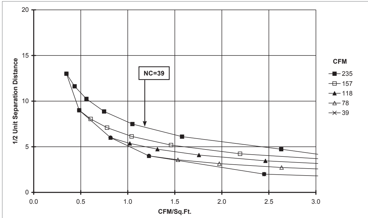
DIFFUSER SPACING FOR 80% ADPI: SHRV, 5SHRV, 18"x18" TO 6" ROUND INLET, 4-WAY (NO DAMPER)
