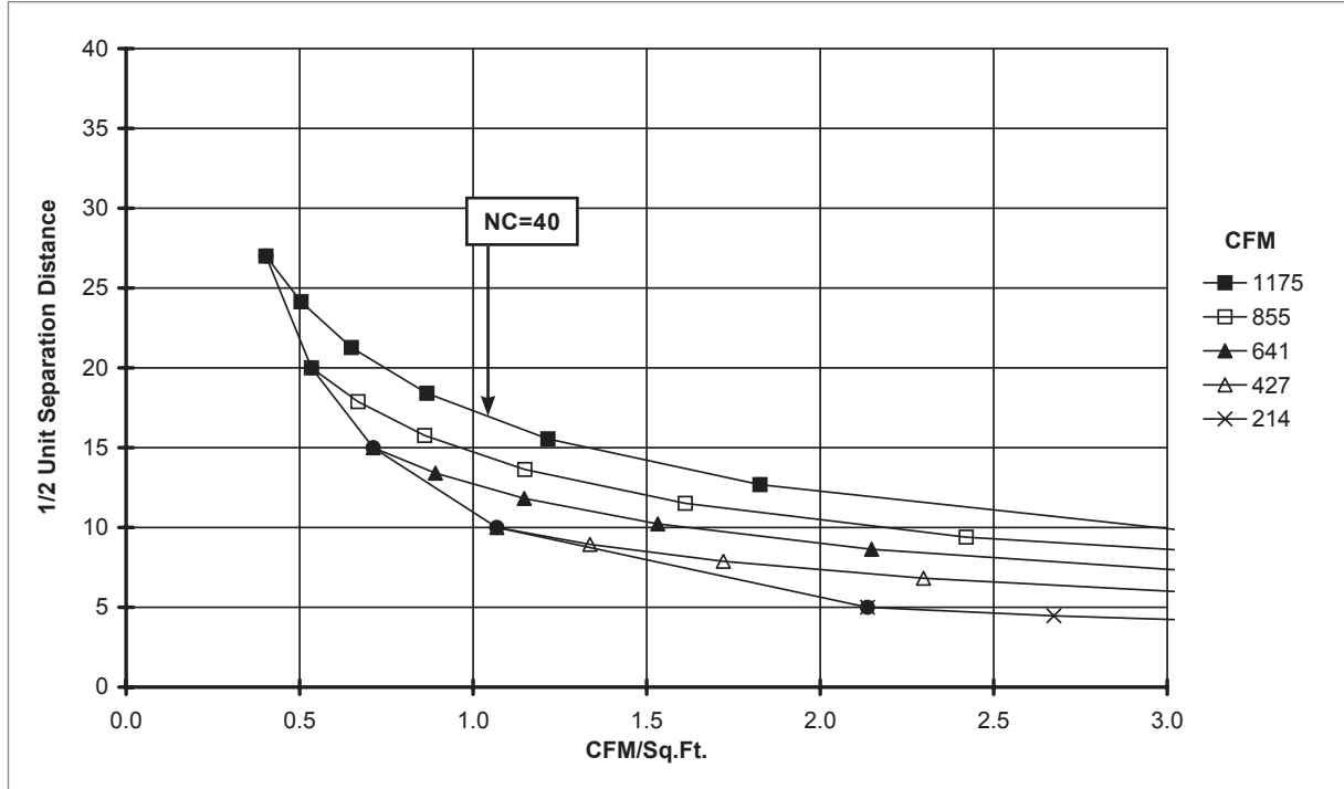
DIFFUSER SPACING FOR 80% ADPI: SHRV, 5SHRV, 18"x18" TO 14" ROUND INLET, 4-WAY (NO DAMPER)
