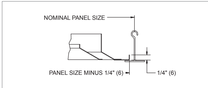
SHR, 5SHR, FRAME 23, LAY-IN T-BAR
