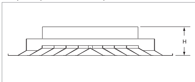
SHR, 5SHR, CROSS SECTION, OVERALL HEIGHT
