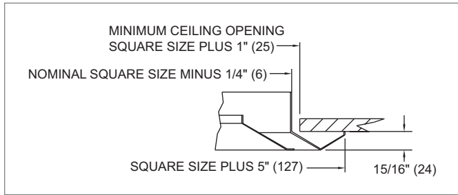
SHR, 5SHR, FRAME 21, SURFACE MOUNT, BEVELED
