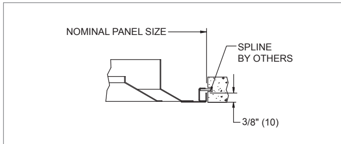
SHR, 5SHR, FRAME 27, SPLINE
