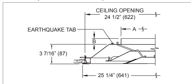
FRAME 22, SURFACE MOUNT, 24"x24" PANEL
