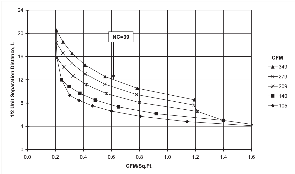
DIFFUSER SPACING FOR 80% ADPI: 1400A, 51400A, 24"x24" PANEL, 8" INLET, 4-WAY (NO DAMPER)
