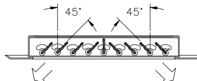
ADJUSTABLE BLADE DETAIL
