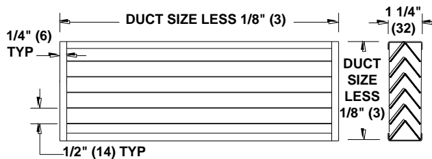
□ MODEL 600C MOUNTING METHOD BY OTHERS
