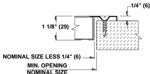
INSTALLATION DETAILS 600
