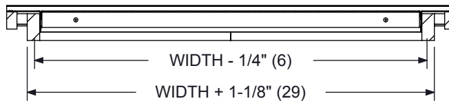
5DMGPU BOTTOM SECTION VIEW
