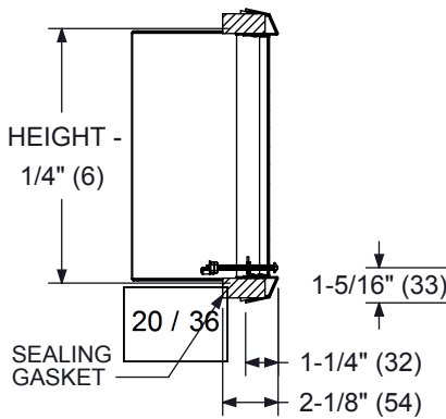
SIDE SECTION VIEW
