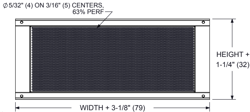
5DMGPU FACE VIEW
