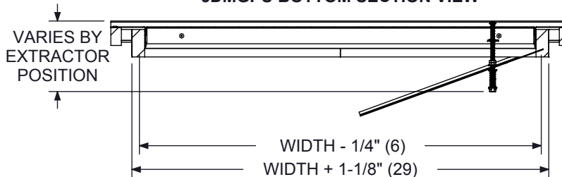
5DMGPU BOTTOM SECTION VIEW
