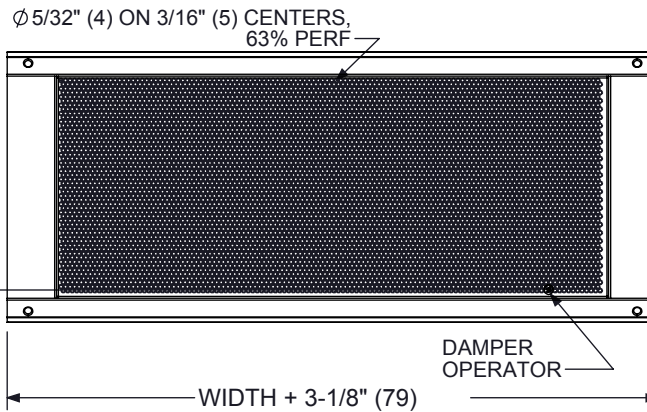
5DMGPU FACE VIEW
