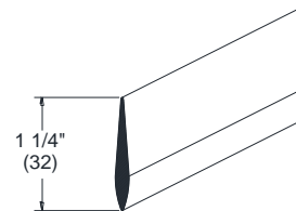
(5)6880-15 BLADE DETAIL
