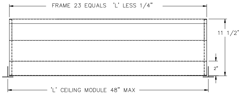
DISCHARGE SIDE VIEW NTS
