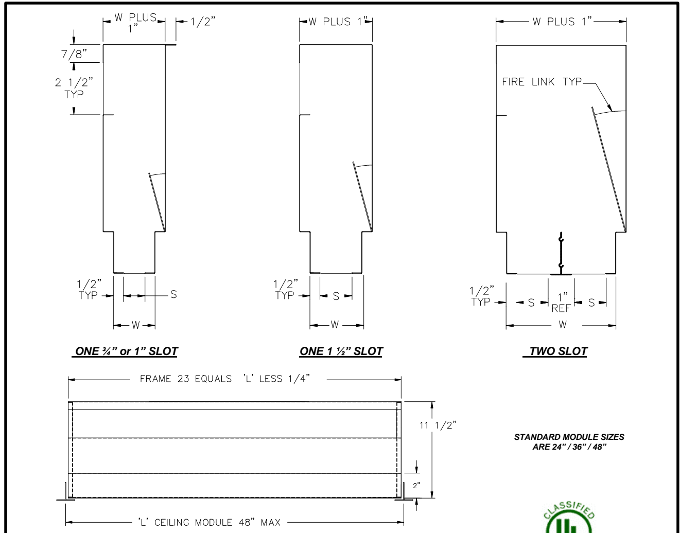
DISCHARGE SIDE VIEW NTS
