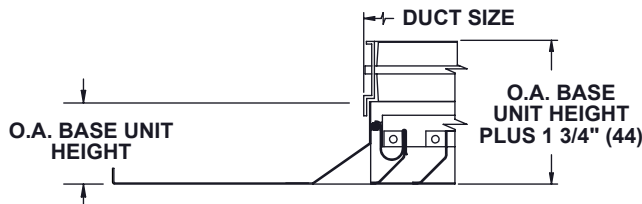
OBD1240 DETAIL TYPICAL OF ALL FRAME STYLES F23 SHOWN
