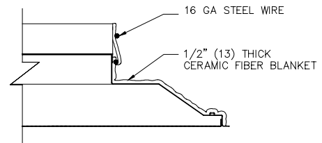
FIRE BLANKET DETAIL
