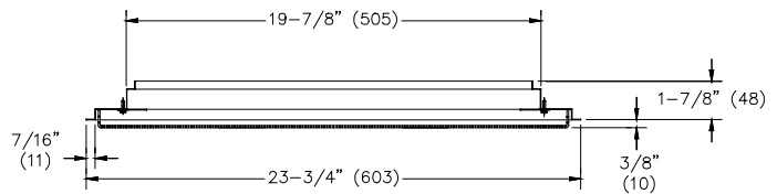
FRAME 30 CROSS SECTION
