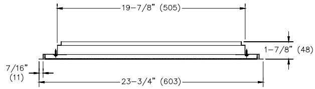
FRAME 23 CROSS SECTION
