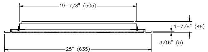
FRAME 20 CROSS SECTION
