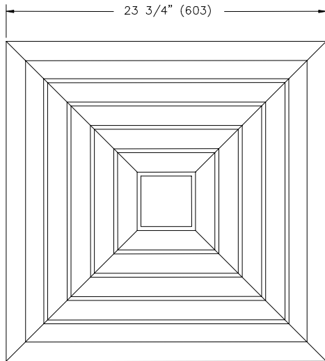
FACE VIEW – FRAME 23
