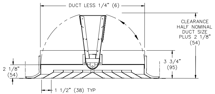
CROSS SECTION
