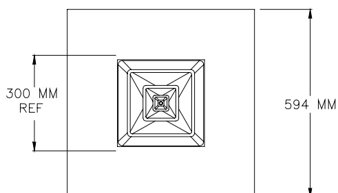
FACE VIEW - FRAME 12 600 x 600
