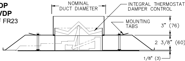
CROSS SECTION
