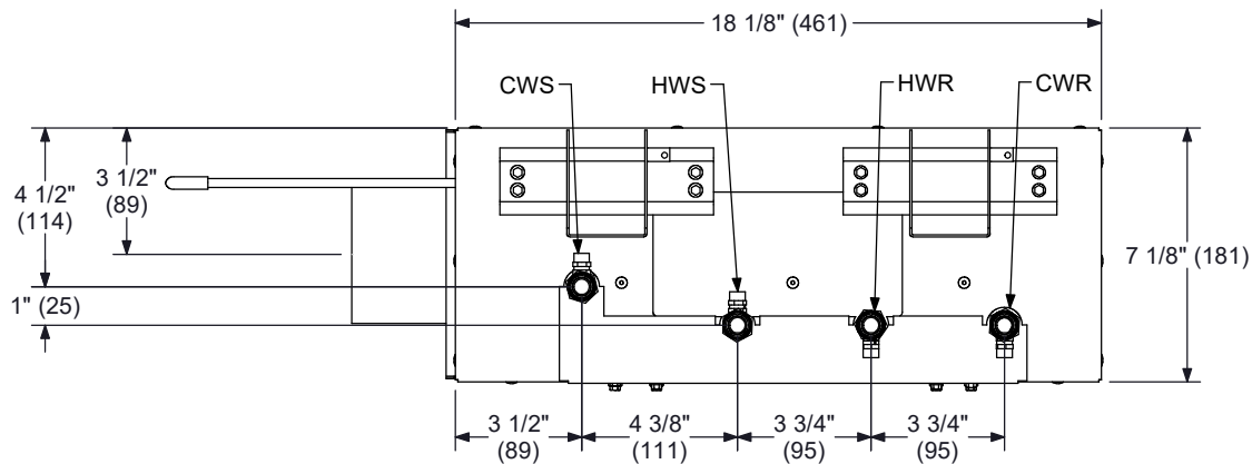
4 PIPE, RIGHT HAND, 2 FT LENGTH SHOWN
