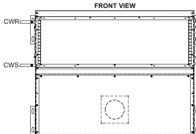
2 PIPE, LEFT HAND, REAR MIDDLE INLET
