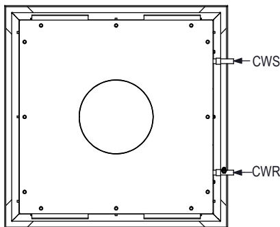
24T, 2 PIPE TOP INLET
