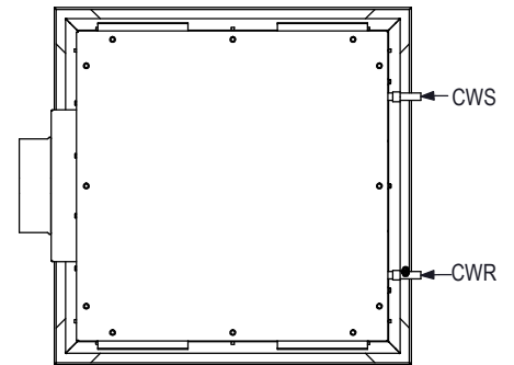
24A, 2 PIPE SIDE INLET
