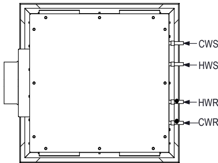
24A, 4 PIPE SIDE INLET
