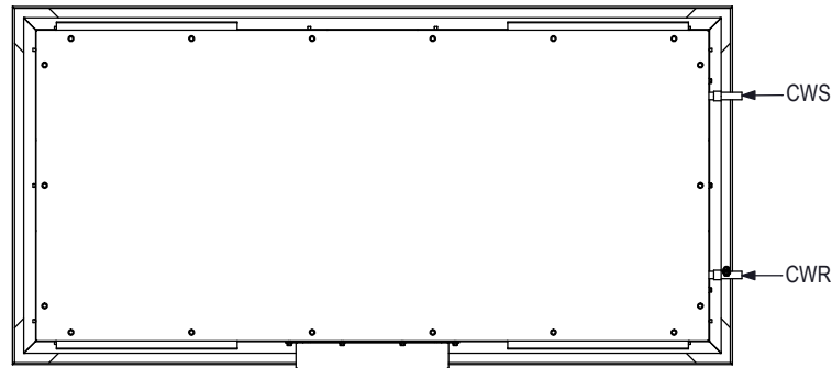
48R, 4 PIPE RIGHT HAND, SIDE INLET
