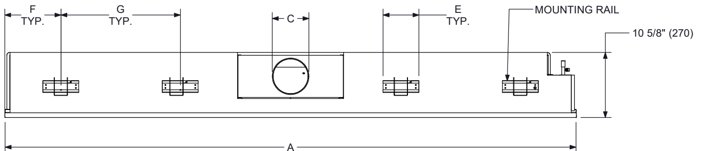
LTF FRAME
