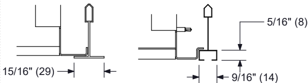
LTF FRAME
