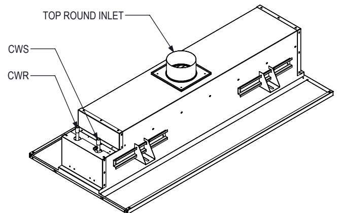
4 PIPE, RIGHT HAND, TOP INLET SHOWN
