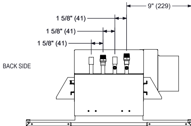
4 PIPE, LEFT HAND, SIDE INLET SHOWN
