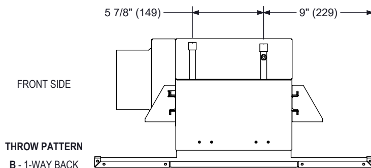
2 PIPE, RIGHT HAND, SIDE INLET SHOWN
