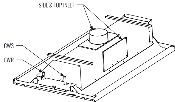
2 PIPE, LEFT HAND, TOP & SIDE INLET SHOWN
