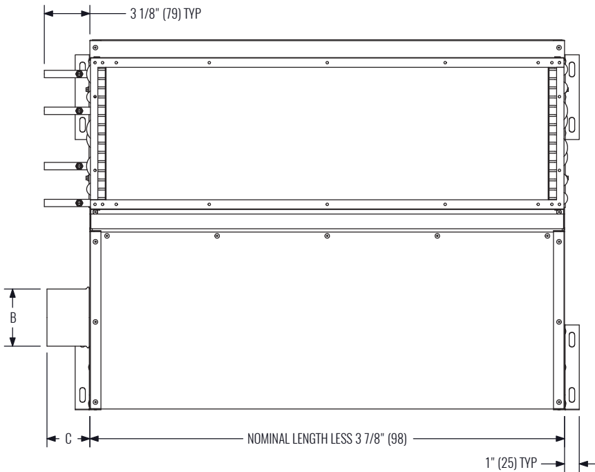
FRONT VIEW
