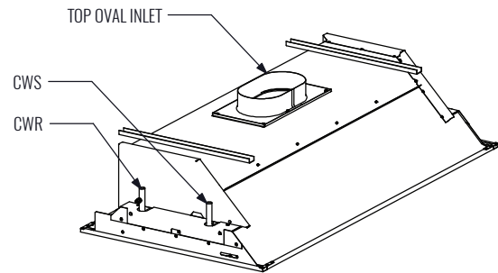
2 PIPE, RIGHT HAND, TOP INLET SHOWN
