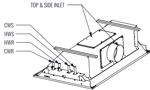
4 PIPE, LEFT HAND, TOP & SIDE INLET SHOWN
